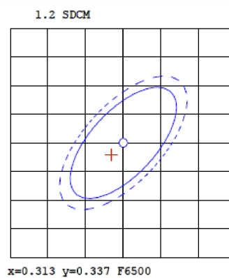
CIE1931 Chromaticity Diagram
